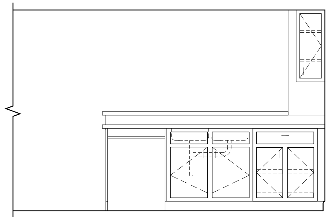
Kitchen Elevations
